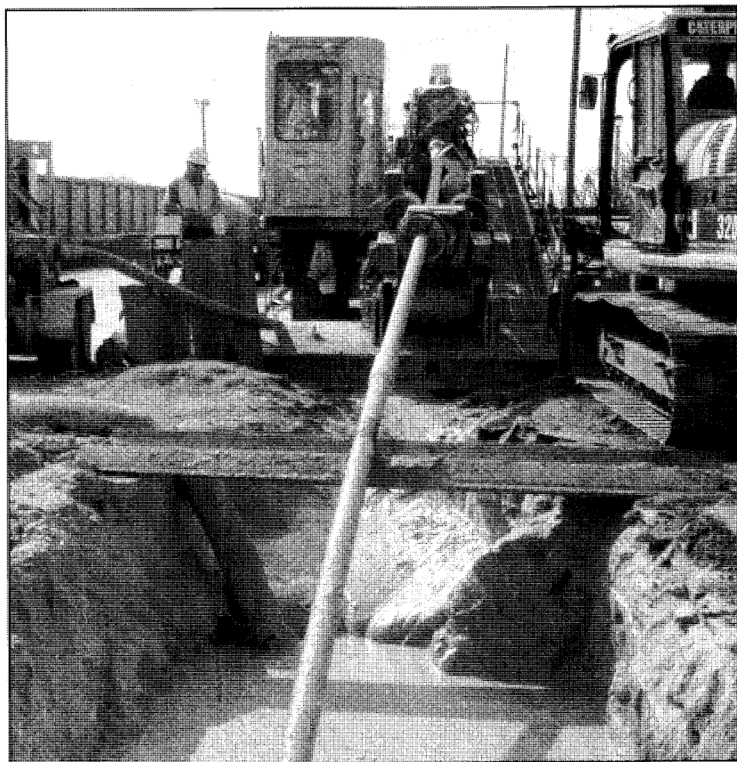
Photos by Staff Sgt. Lonnie Woods Thomas Dean, a supervisor with Big Warrior Corporation, watches as a horizontal boring machine drills a pilot hole more than 3,000 feet while installing a new water main on Main Post near the MP Station. The technology allows pipes to be installed under roads without digging trenches or disrupting the flow of traffic.
