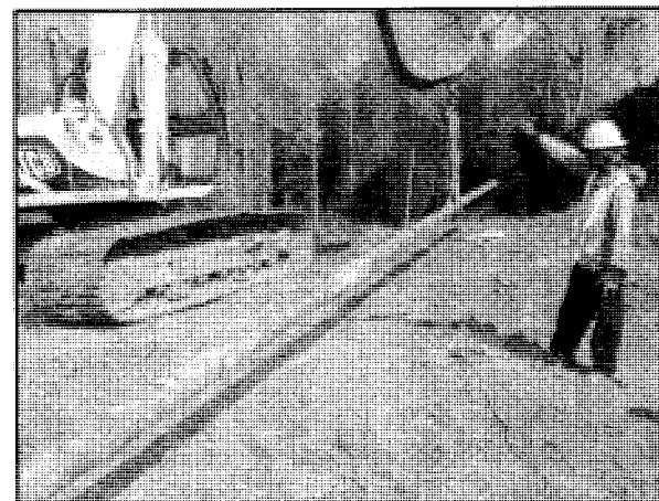
A large diameter auger will be pulled back through the pilot hole to increase its size. The thick walled plastic water pipe will then be pulled through the enlarged hole and joined to existing pipe.
